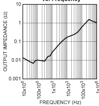
D2632 Output Impedance vs. Frequency
