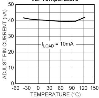
D2632 Adjust Pin Current vs. Temperature
